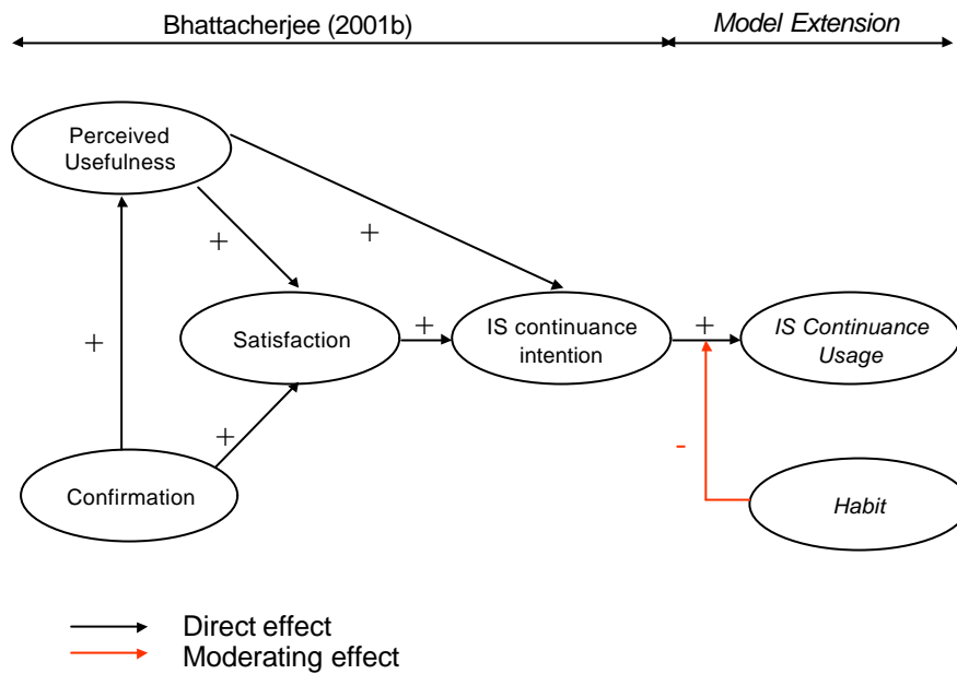
Figure 1: Extended research model, based on (Bhattacherjee 2001)
