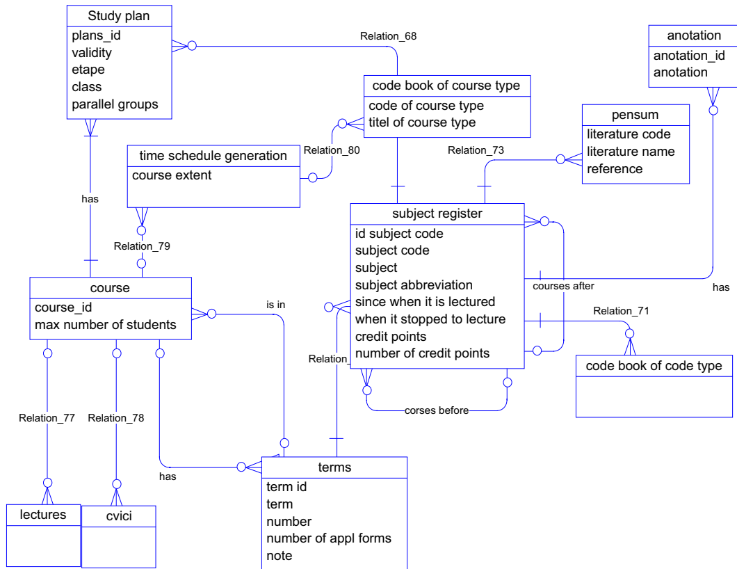
Fig. 2: Part of data conceptual model
