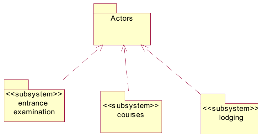
Fig. 3: Package diagram of new PIS version
